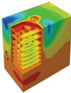
Deep excavation
