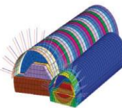
Construction stage
